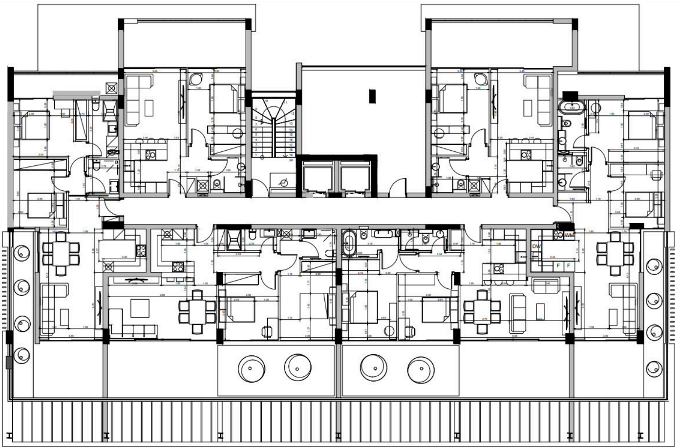
1ST FLOOR PLAN AS PROPOSED
